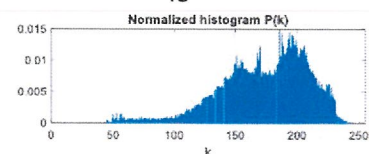
H3
